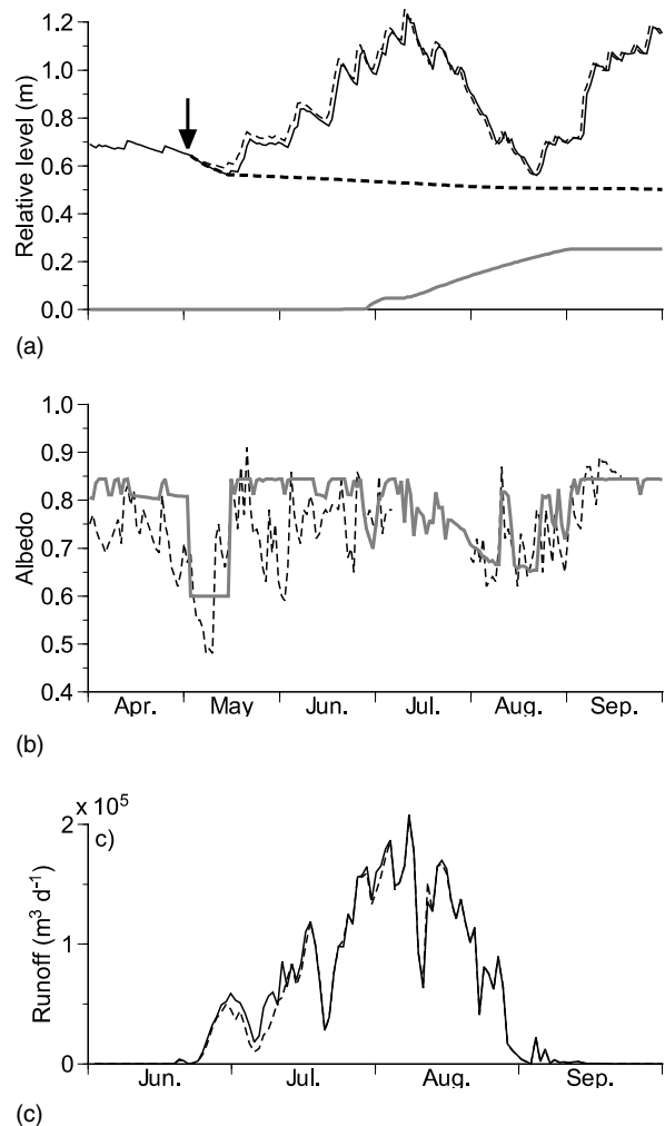
Figure 3. (a) Relative levels of surface (solid line), dusted layer (thick broken line), and snow-ice interface (grey line) at 5600 m a.s.l. of Xiao Dongkemadi Glacier when surface was dusted on 2 May in the calculation (arrow). Surface level of the control run is shown as a thin broken line for comparison. (b) Observed and calculated albedos (broken and grey lines in denote respectively). (c) Calculated runoff (solid line) differs slightly from the control result (broken line)
