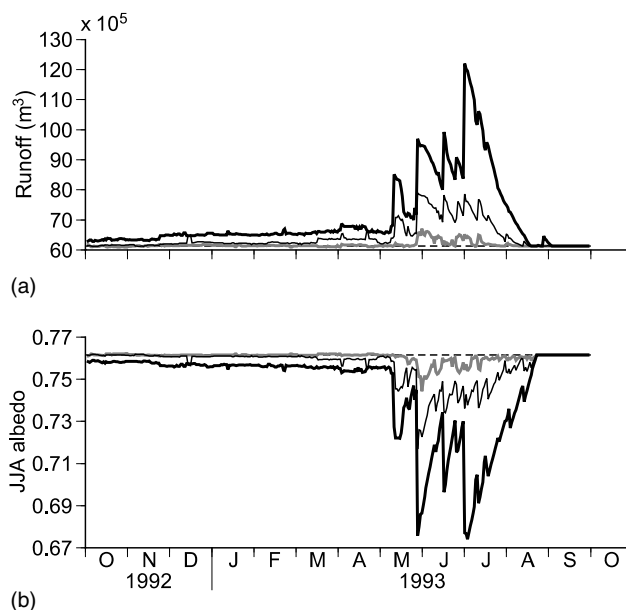
Figure 5. Seasonal sensitivities of (a) glacier runoff on the changes in dusted date and albedo and (b) summer mean albedo of the glacier. Horizontal and vertical axes denote the dusted date and total glacier runoff (a) and summer mean albedo (b) respectively. Thick, thin, and grey lines denote albedos of dusted surface as 0.7, 0.6 and 0.5 respectively. Runoff amount and summer mean albedo of the control calculation ( 61.3 \times 10^5 \text{ m}^3 and 0.762 respectively) are shown as straight broken lines
