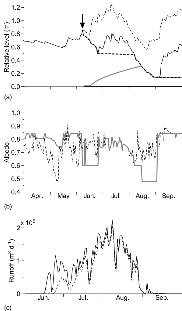
Figure 4. (a) Relative levels of surface (solid line), dusted layer (thick broken line), and snow-ice interface (gray line) at 5600 m a.s.l. of Xiao Dongkemadi Glacier when surface was dusted on 6 June in the calculation (arrow). Surface level of the control run is shown as a thin broken line for comparison. (b) Observed and calculated albedos (broken and grey lines in denote respectively). (c) Calculated runoff (solid line) differs obviously from the control result (broken line)
