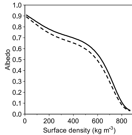
Figure 1. Albedos of dry (solid line) and wet (broken line) snow versus surface snow density
