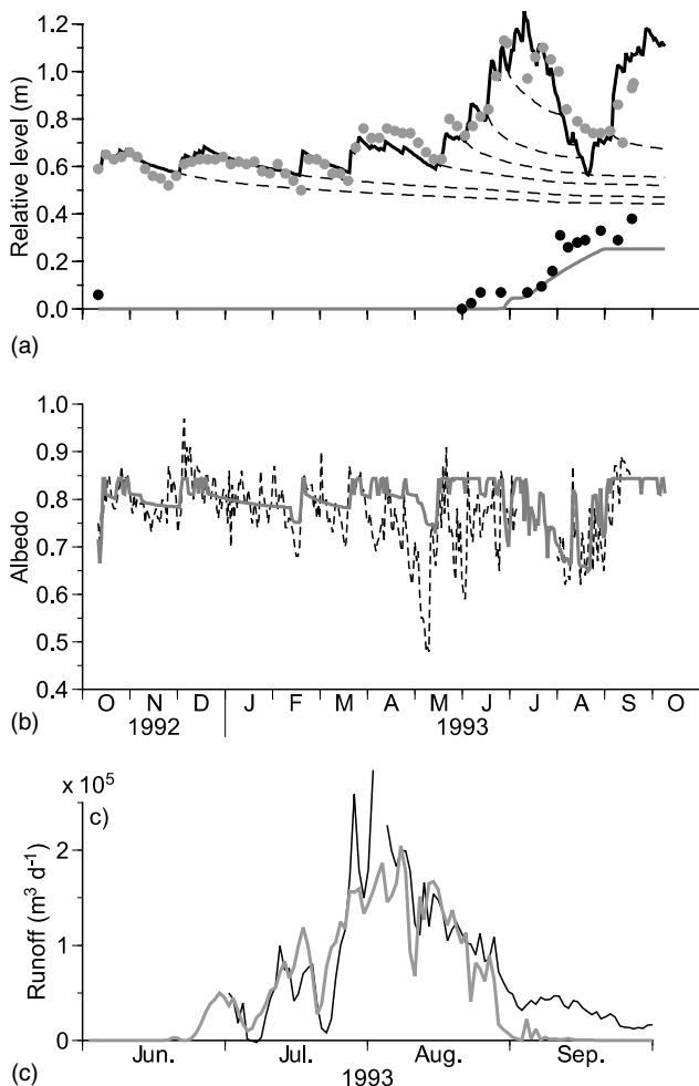
Figure 2. (a) Relative levels of surface (solid line), dirt layers (broken lines), and snow-ice interface (grey line) at 5600 m a.s.l. of Xiao Dongkemadi Glacier. Observed surface (grey circles) and snow-ice interface (black circles) are compared with those calculated. (b) Observed (broken line) and calculated (grey line) albedos at the same elevation. (c) Calculated runoff (grey line) accurately represents the estimated runoff (solid line) from observation. A more detailed description is shown in Fujita et al. (in press)
