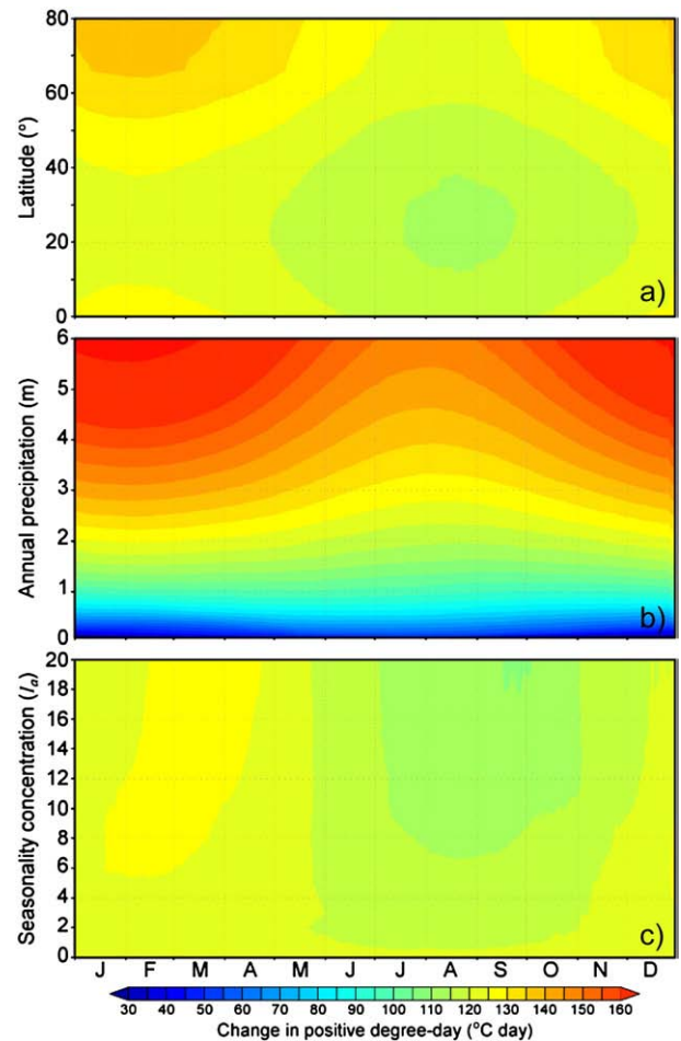
Fig. 4. Change in positive degree-day sum at the ELA to uniform warming (+1 °C). a) Effect of latitude under a given annual precipitation (2 m w.e.) with a given concentration ( I_a=6 ). b) Effect of annual precipitation with a given concentration ( I_a=6 ) at a given latitude (40°). c) Effect of seasonality concentration under a given annual precipitation (2 m w.e.) at a given latitude (40°). Abscissa denotes the date of maximum precipitation in all panels.
