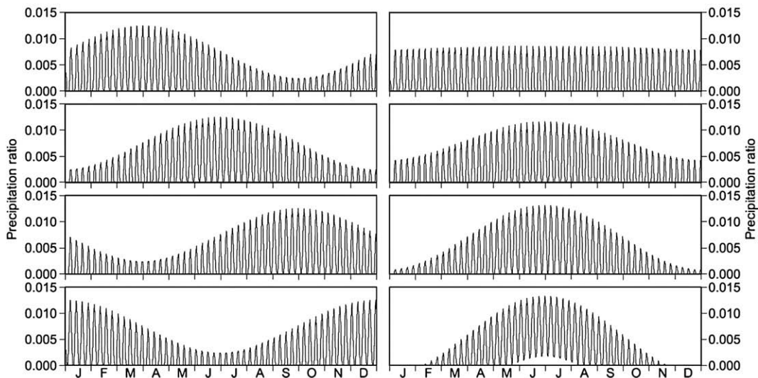
Fig. 2. Examples of precipitation pattern. Left panels show changes in the date of maximum precipitation ( d_{\max}=91, 182, 273, 364 , top to bottom) with a given seasonality concentration ( I_a=4 ). Right panels show changes in seasonality concentration ( I_a=0, 4, 8, 12 , top to bottom) with a given date of the maximum precipitation ( d_{\max}=182 ).
