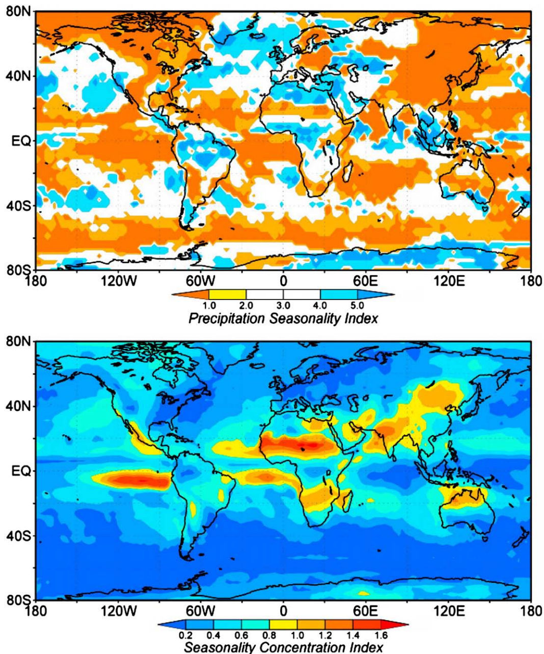
Fig. 5. Distribution of precipitation seasonality index (PSI, upper) and seasonality concentration index (SCI, lower). See text for the definition.
