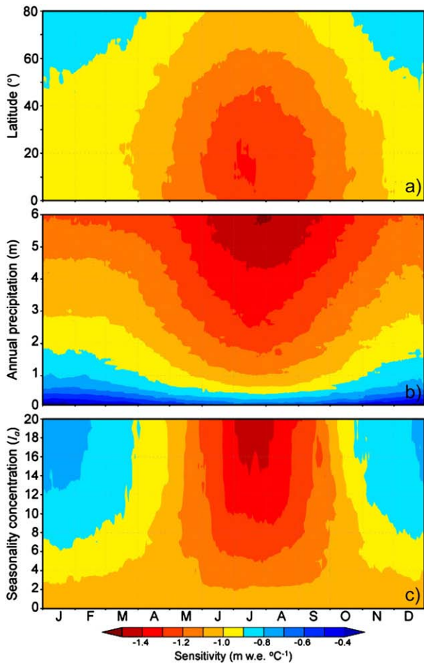
Fig. 3. Climatic sensitivity of glacier mass balance to uniform warming (+1 °C). a) Effect of latitude under a given annual precipitation (2 m w.e.) with a given concentration ( I_a=6 ). b) Effect of annual precipitation with a given concentration ( I_a=6 ) at a given latitude (40°). c) Effect of seasonality concentration under a given annual precipitation (2 m w.e.) at a given latitude (40°). Abscissa denotes the date of maximum precipitation in all panels.
