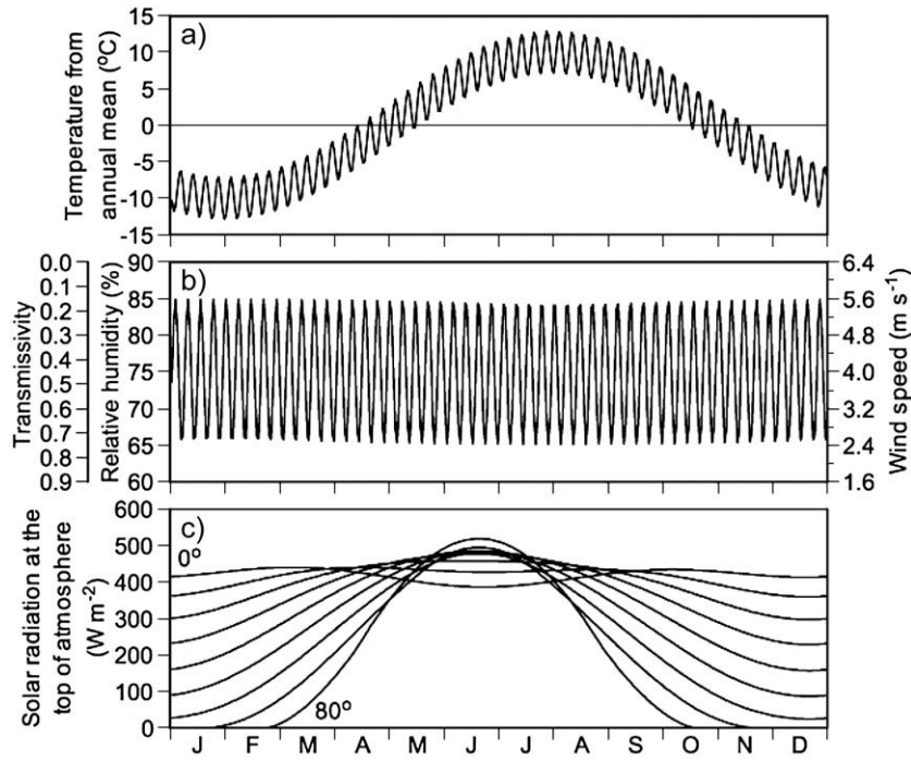
Fig. 1. Simplified meteorological variables for the model: (a) air temperature; (b) wind speed, relative humidity and transmissivity for solar radiation, expressed by a single curve with different ordinate axes; and (c) solar radiation at the top of the atmosphere. Multiplying solar radiation at the top of the atmosphere, which is obtained at each latitude, by the transmissivity gives the solar radiation at the surface.
