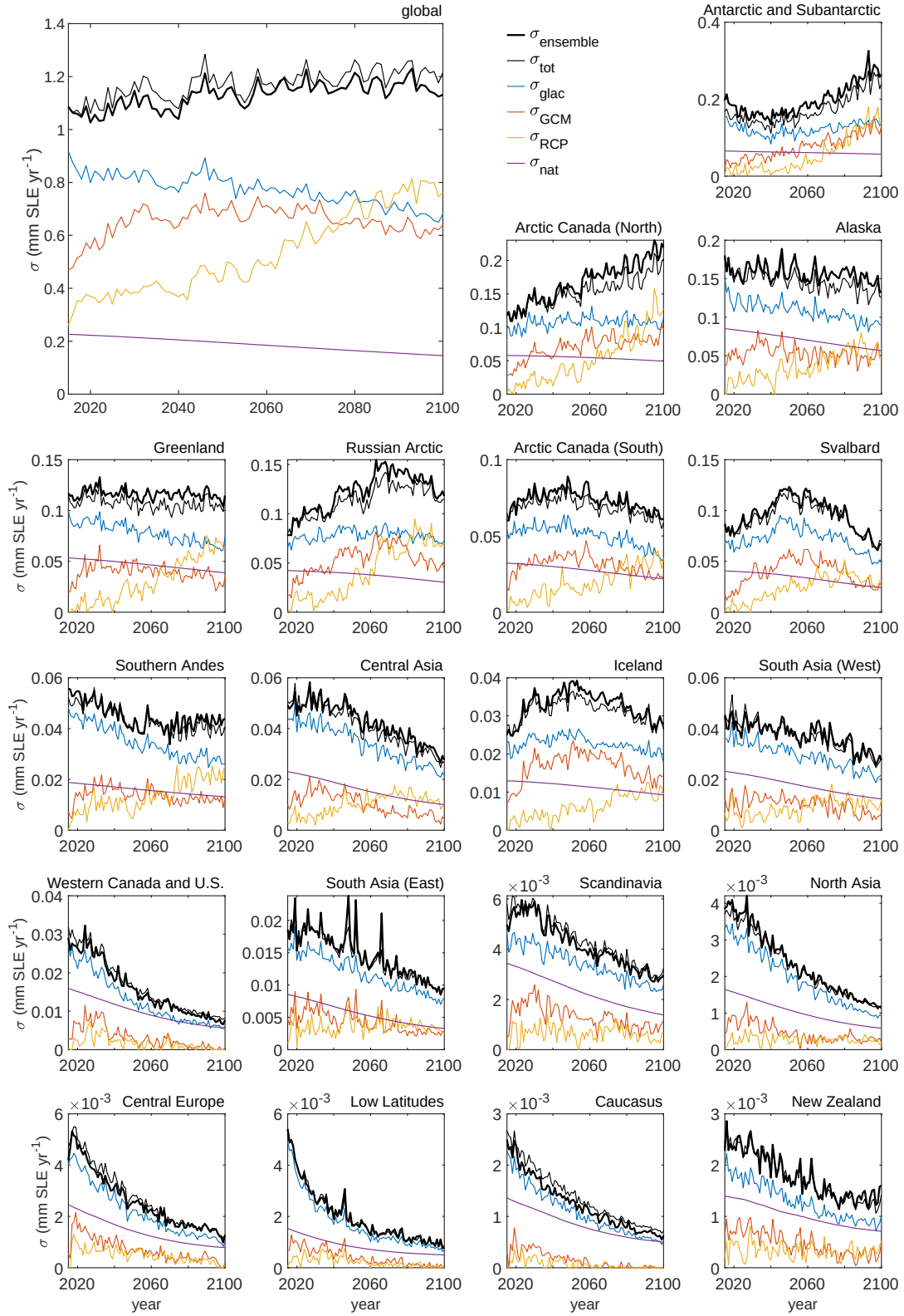
Figure S21 Contribution of each source of uncertainty (Equations 3-6) to the total uncertainty ( \sigma_{\text{tot}} , Equation 2) of projected mass loss rates in \text{mm SLE yr}^{-1} . Also shown is the uncertainty obtained directly from the entire ensemble without any decomposition ( \sigma_{\text{ensemble}} ).
