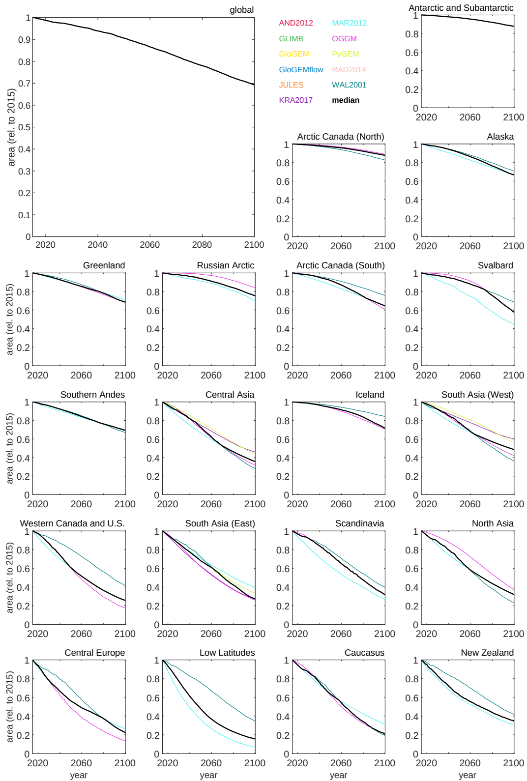
Figure S7 As Fig. S5, but for scenario RCP6.o.
